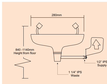
Eyewash with ABS Bowl Model : EY 5050
